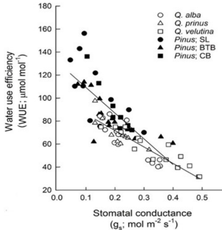
Figure 7: Inverse correlation between water use efficiency (WUE, \mu\text{mol CO}_2 captured per mol \text{H}_2\text{O} lost), and stomatal conductance ( g_s ; \text{mol H}_2\text{O m}^{-2} \text{s}^{-1} ) for oaks ( Quercus , y = -143x + 100.3 ; r^2 = 0.79 ) and pines ( Pinus , y = -224x + 131.6 ; r^2 = 0.54 ), Renninger et al. (2013), Fig. 3, adapted [55]. In this experiment, the reduction of stomatal conductance was drought induced. However, we also observe a reduced stomatal conductance under e\text{CO}_2 , when a higher photosynthetic rate even more enhances water use efficiency.
