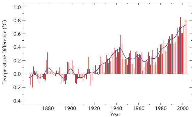
Observed global average land temperatures relative to the end of the 19th century
