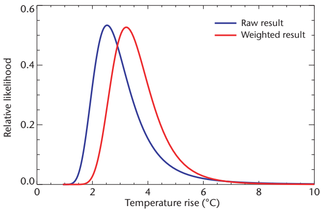
Global average annual warming predicted by a 53-member model ensemble for a doubling of atmospheric carbon dioxide concentrations
