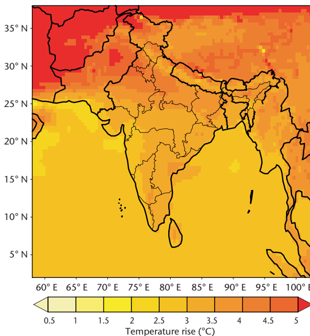
The predicted change in Jun–Sept temperature between the present day and the 2080s, for the SRES A2 scenario
