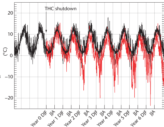
Predicted daily minimum CET following an artificial shutdown of the THC. The black curve shows the climate with no THC shutdown. The red curve shows the result after THC shutdown
