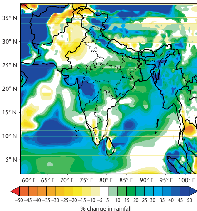
The predicted percentage change in Jun–Sept precipitation between the present day and the 2080s, for the SRES A2 scenario
