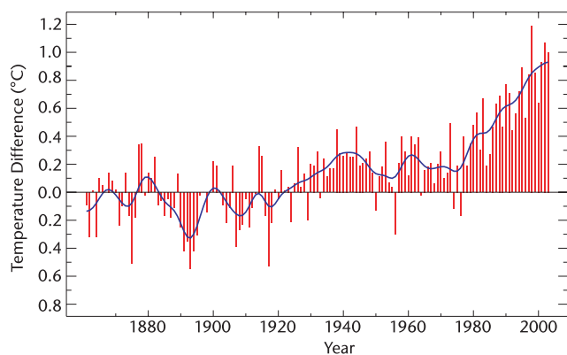
Observed global average land temperatures relative to the end of the 19th century
