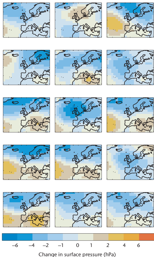
Predicted change in surface pressure over Europe from a subset of the model versions used to generate likelihood predictions
